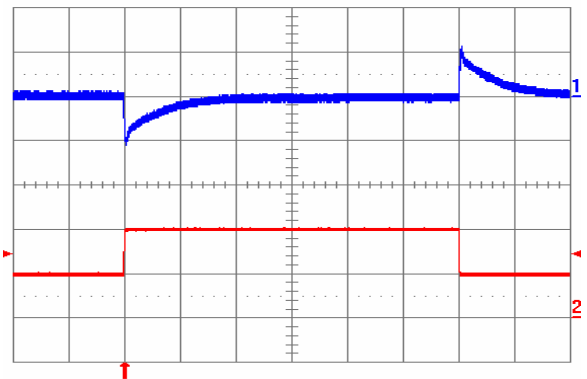
Fig. 21: Output voltage response to load current step-change (5 A – 10 A – 5 A) at V_{in} = 48\text{ V} . Top trace: output voltage (100 mV/div). Bottom trace: load current (5 A/div). Current slew rate: 5 A/ \mu\text{s} . C_o = 450\ \mu\text{F} tantalum + 1 \mu\text{F} ceramic. Time scale: 0.2 ms/div.
