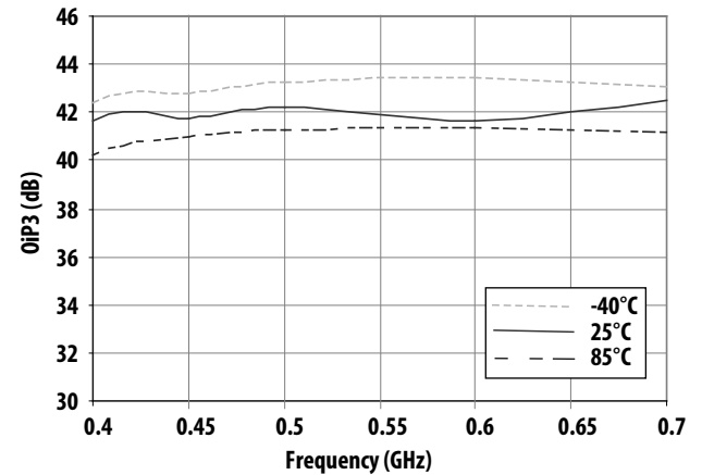
Figure 25. Over Temperature OIP3 vs Frequency
