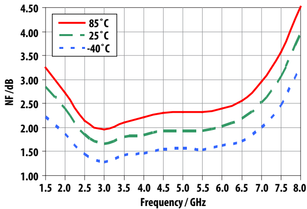
Figure 7. Noise Figure vs Frequency
