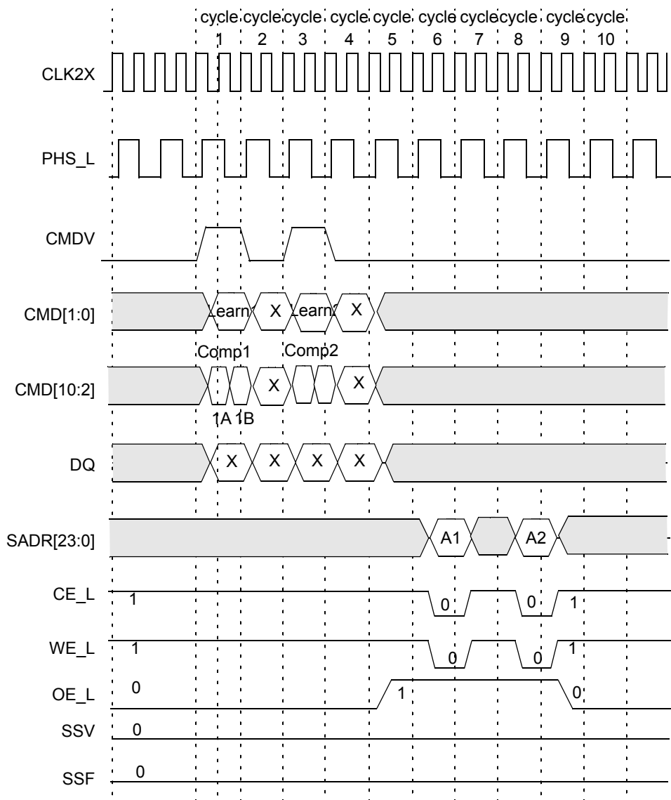
Figure 10-73. Timing Diagram of Learn (TLSZ = 00)
