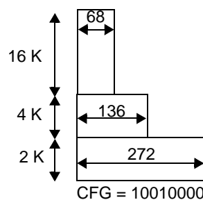
Figure 10-72. Multiwidth Configurations Example
