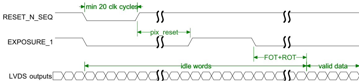
Figure 34. Sequencer Reset
