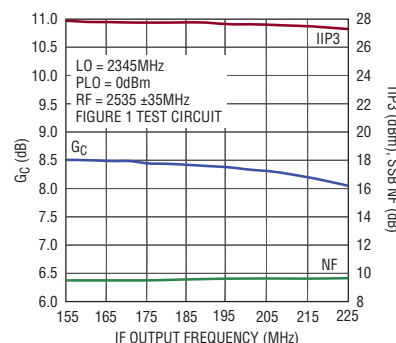
Wideband Conversion Gain, IIP3 and NF vs IF Frequency (Mixer Only, Measured on Evaluation Board)
