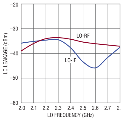
LO Leakage vs LO Frequency
