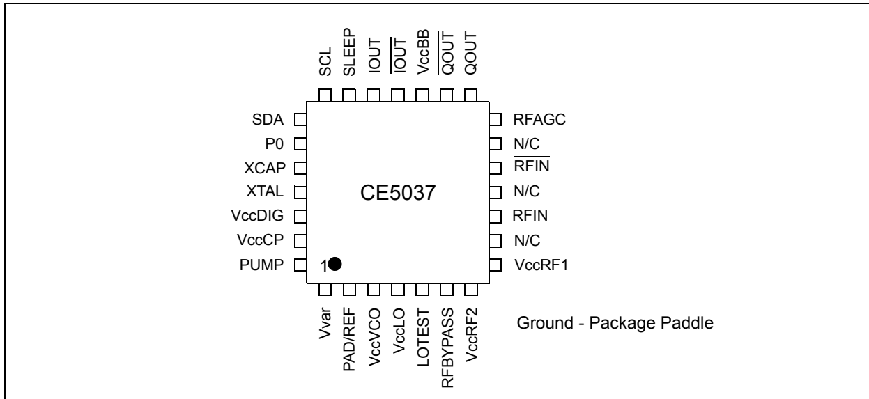
Figure 2 - Pin Diagram
