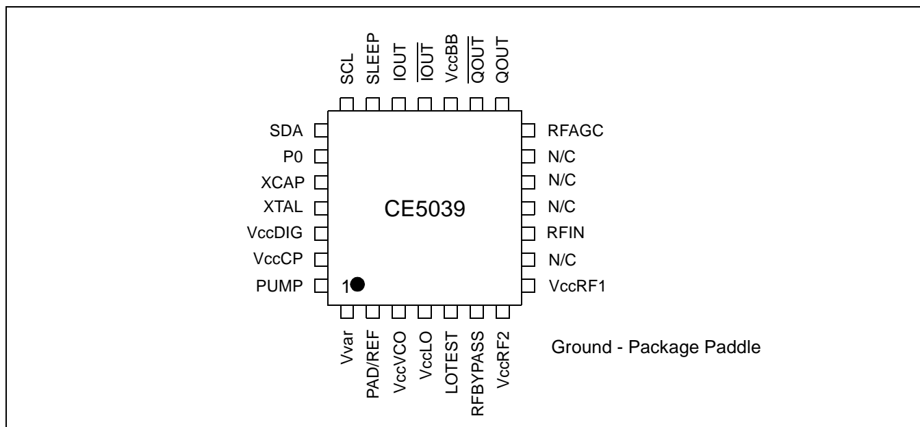
Figure 2 - Pin Diagram
