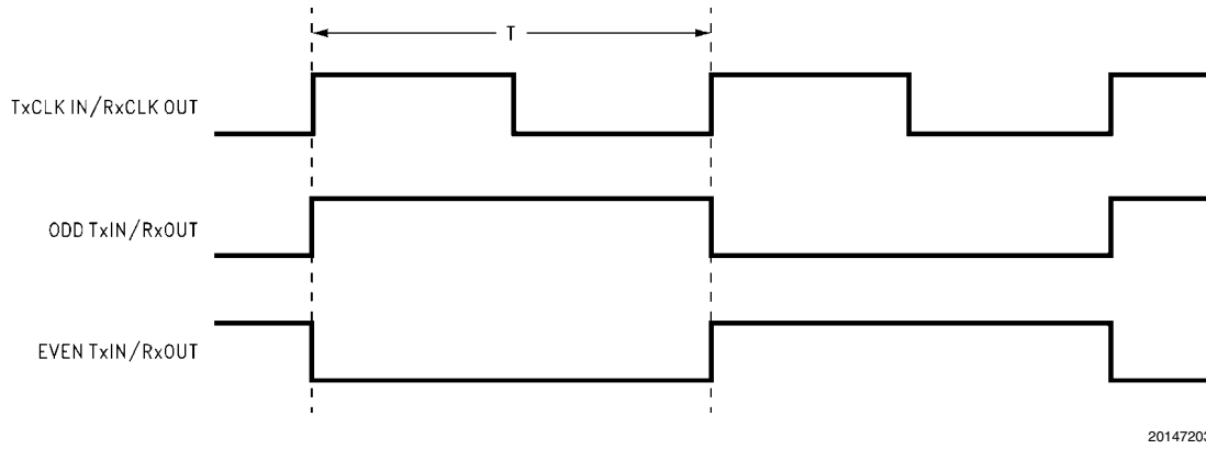
FIGURE 2. "Worst Case" Test Pattern
