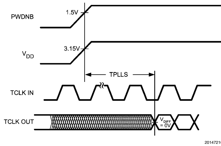
FIGURE 8. Phase Lock Loop Set Time
