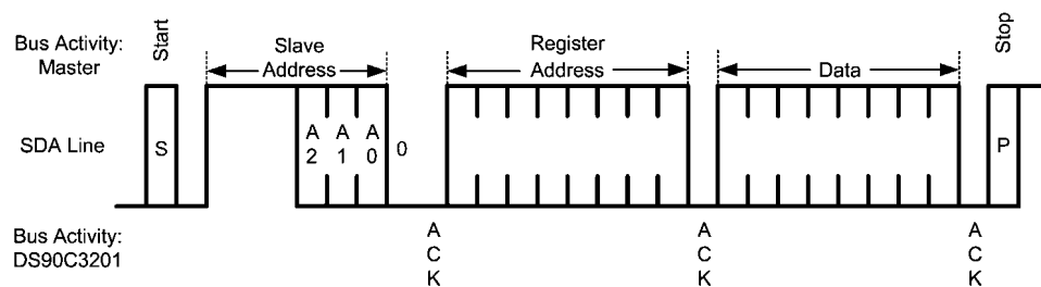
FIGURE 15. Byte Write
