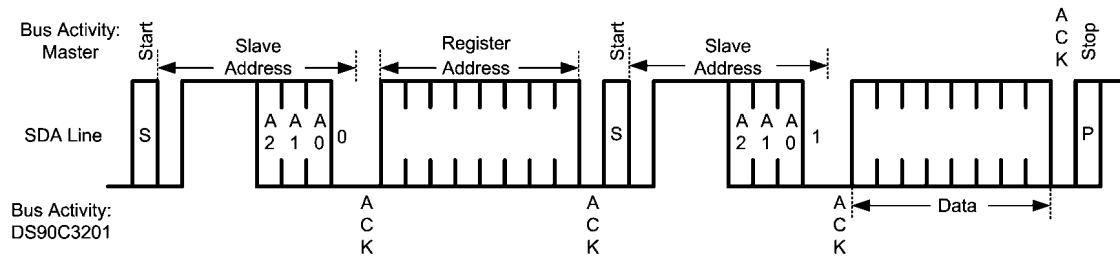
FIGURE 14. Byte Read
