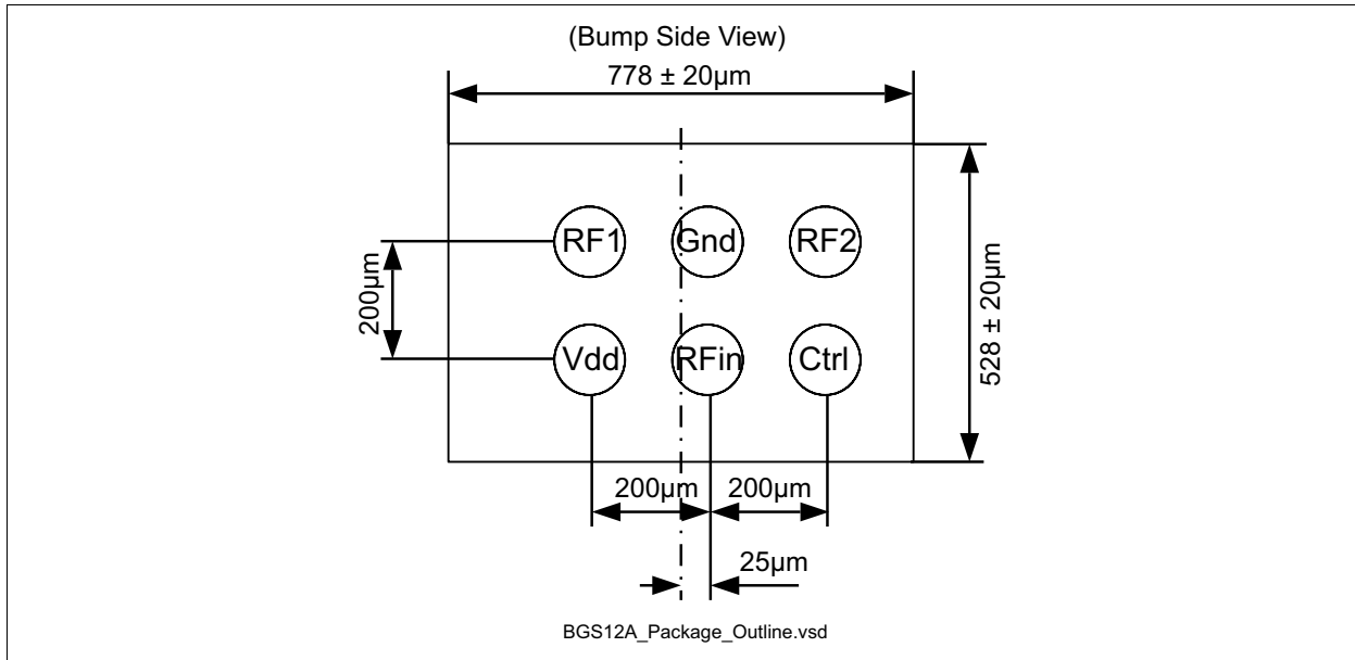
Figure 3 Package outline
