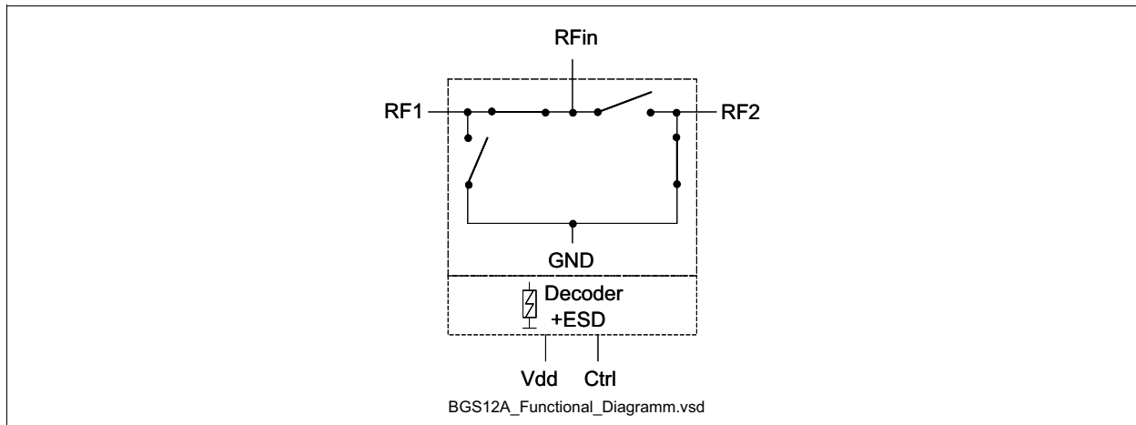
Figure 1 Functional Diagram
