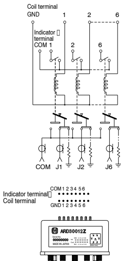
Fail-safe type
