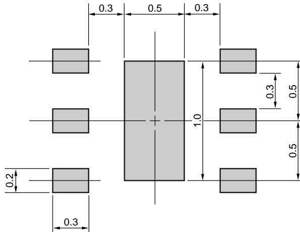
MOUNTING PAD
