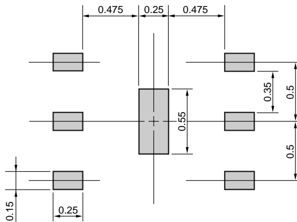
SOLDER PAD
