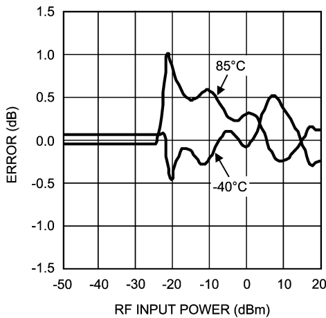
Output Variation vs. RF Input Power Normalized to 25°C @ 900 MHz (LMV226)
