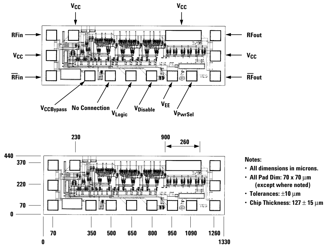
Figure 2. Pad Locations and Chip Dimensions.
