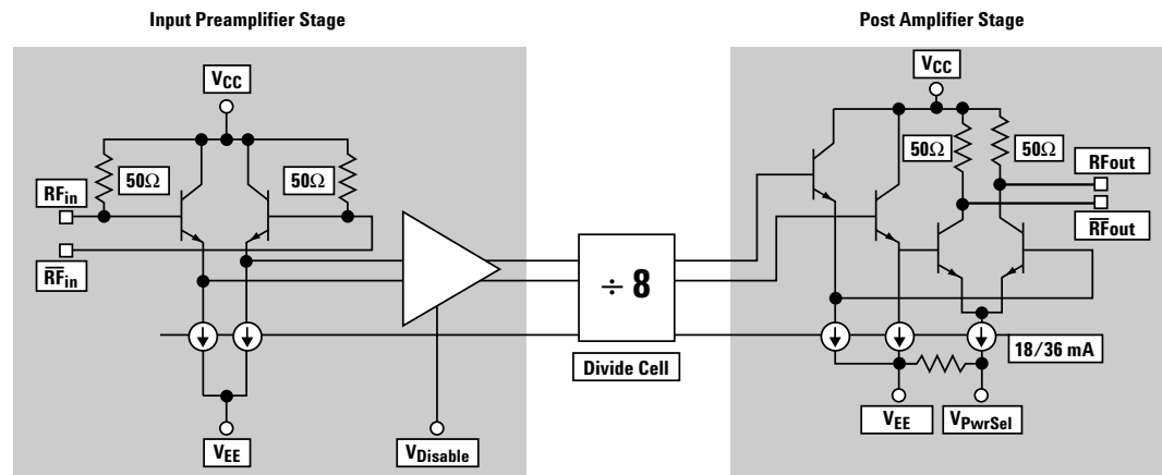
Figure 1. HMMC-3028 Simplified Schematic.
