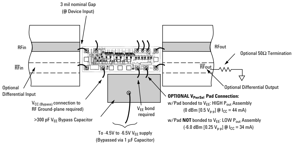
Figure 3. Assembly Diagrams.
