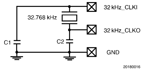
FIGURE 8. 32.768 kHz Oscillator
