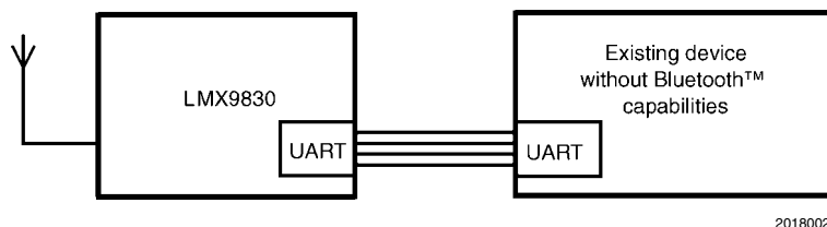
FIGURE 15. Bluetooth Functionality
