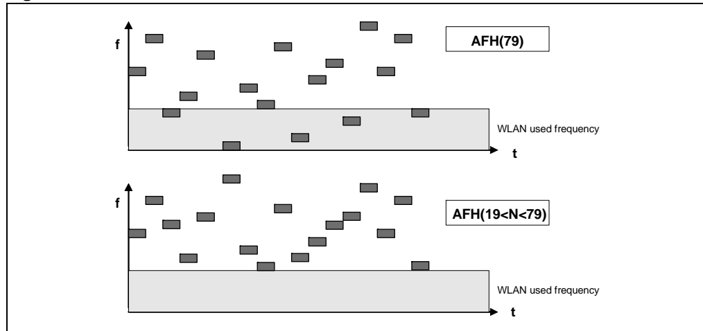
Figure 5. AFH
