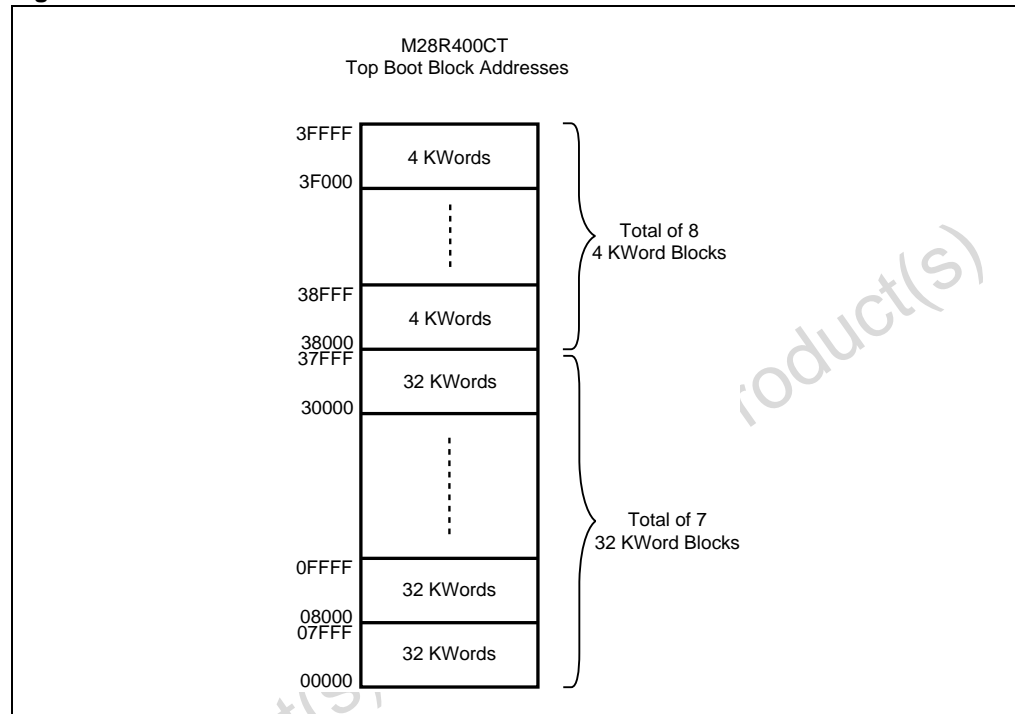
Figure 3. Block addresses
