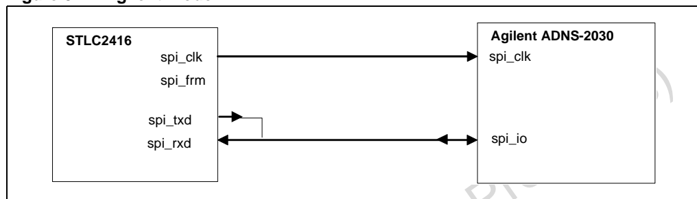
Figure 9. Agilent mode
