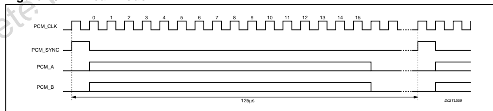
Figure 13. Linear mode
