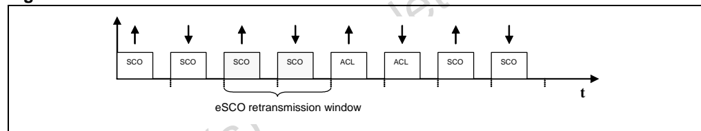
Figure 4. Extended eSCO
