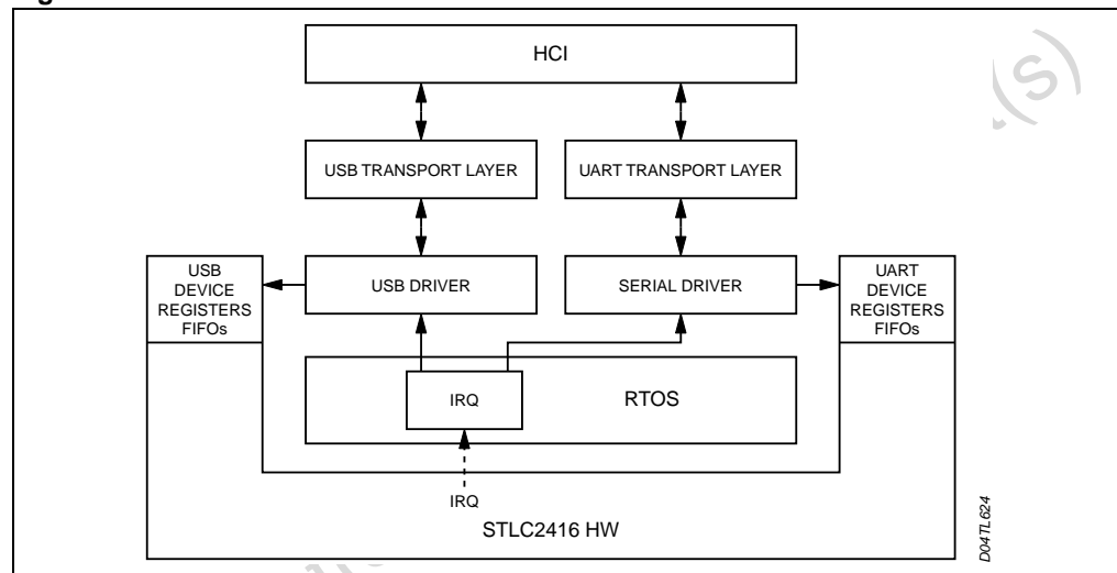
Figure 11. USB interface
