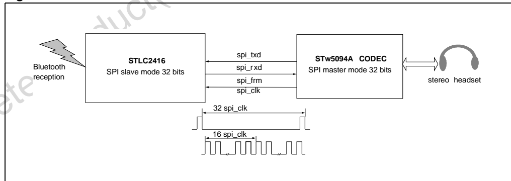
Figure 10. 32-bit SPI
