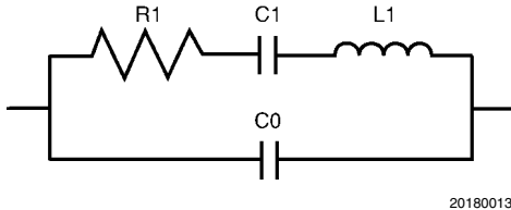
FIGURE 5. Crystal Equivalent Circuit
