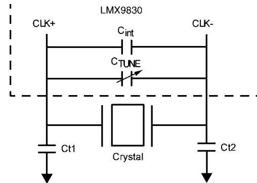
FIGURE 4. LMX9830 Crystal Recommended Circuit
