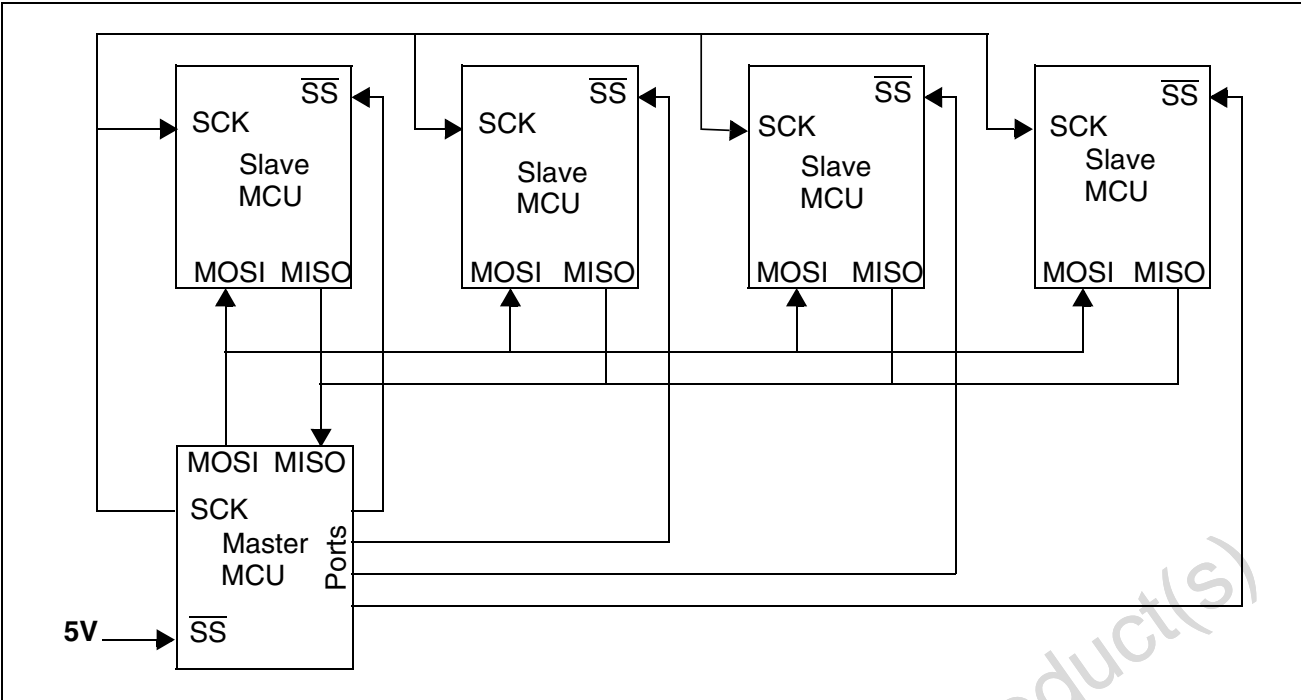
Figure 15.6 Single Master Configuration
