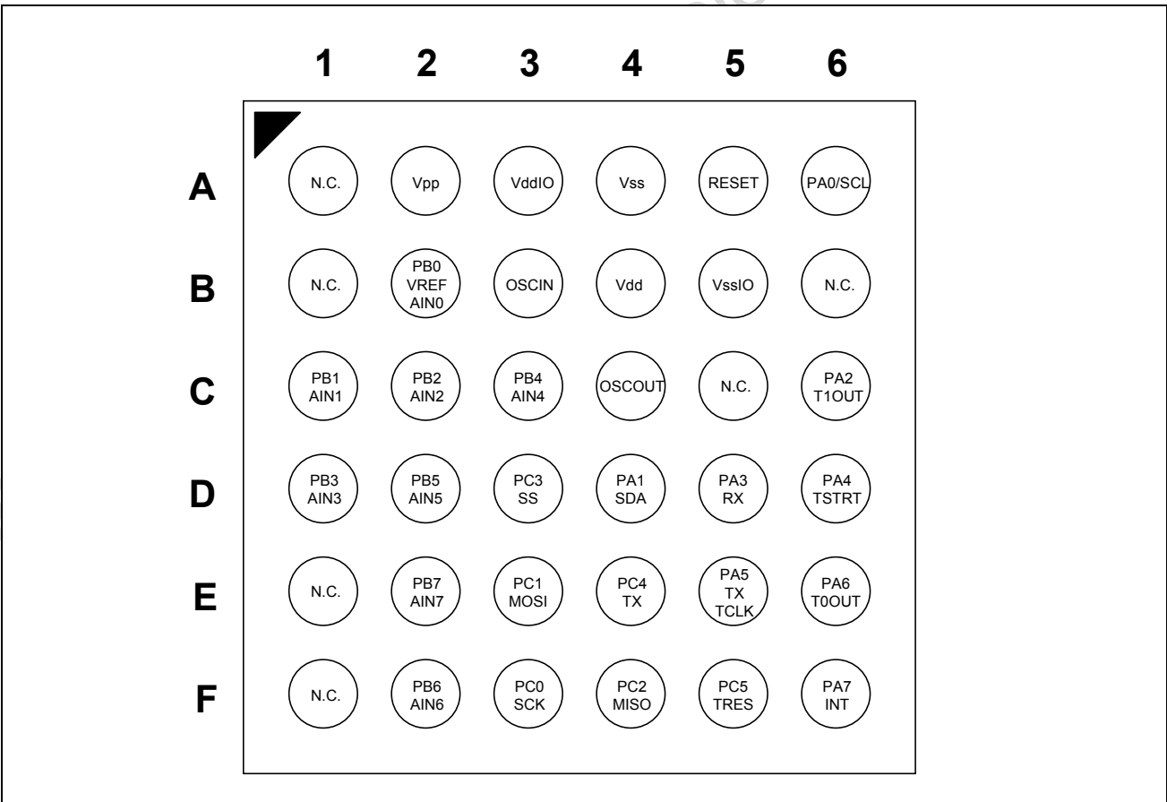
Figure 1.5 ST52510/513 LFBGA36 Pin Configuration (view through package)
