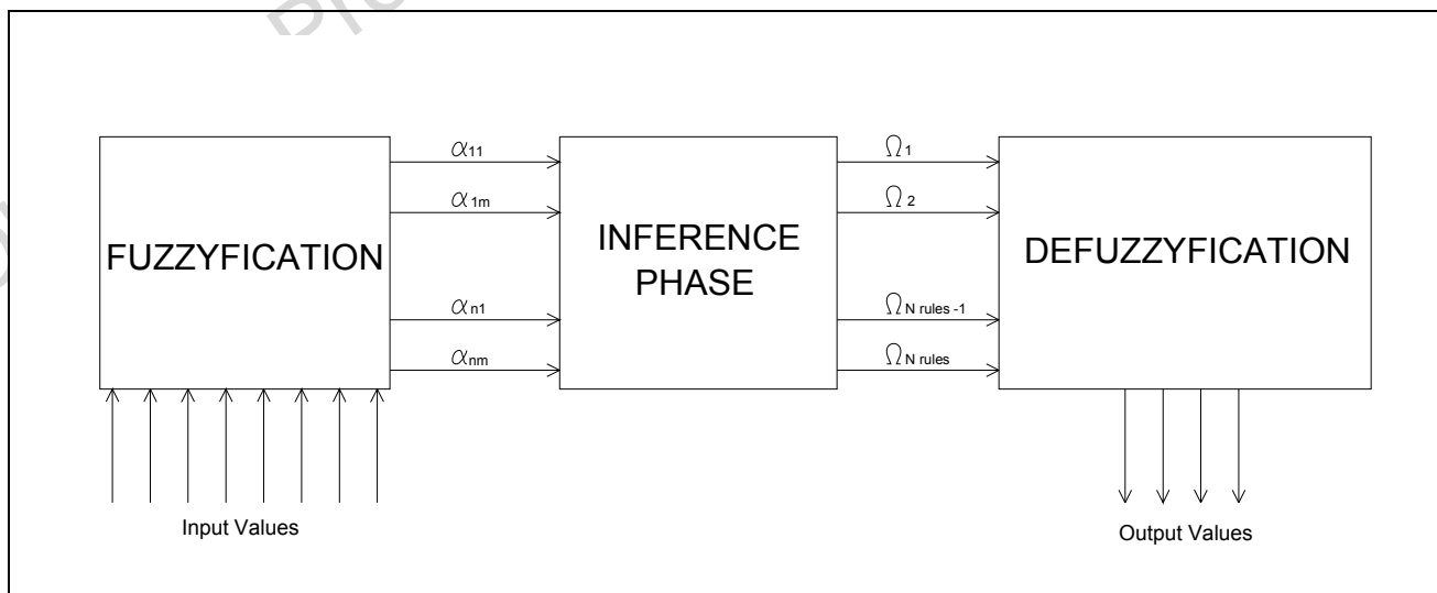
Figure 8.1 Fuzzy Inference
