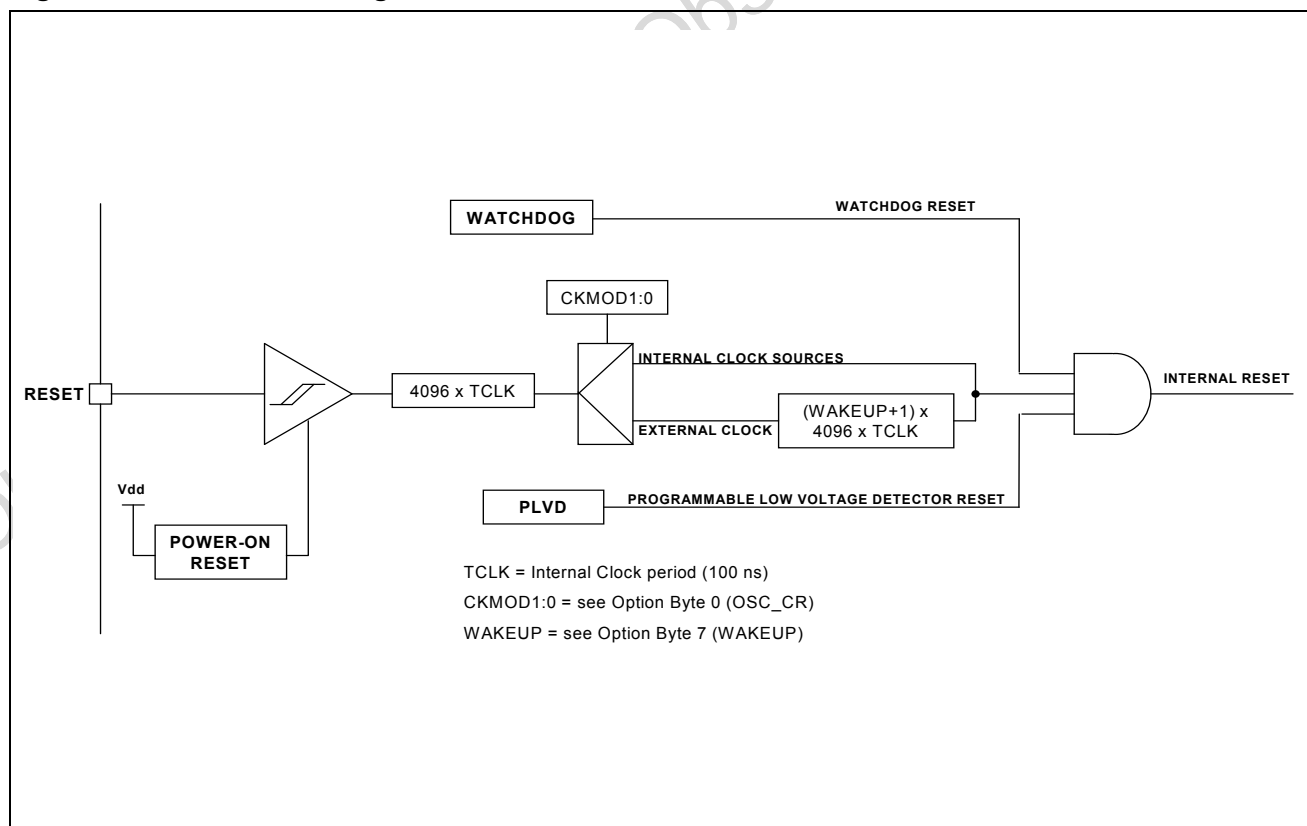
Figure 6.2 Reset Block Diagram
