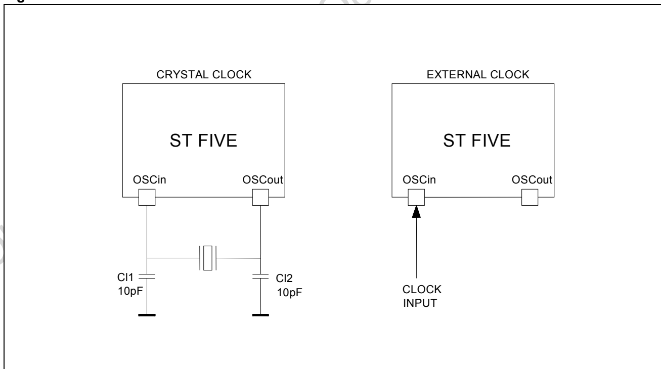
Figure 6.1 Oscillator Connections
