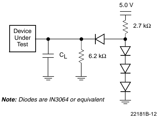
Figure 7. Test Setup
