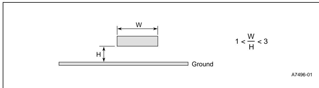
Figure 5. Trace Geometry
