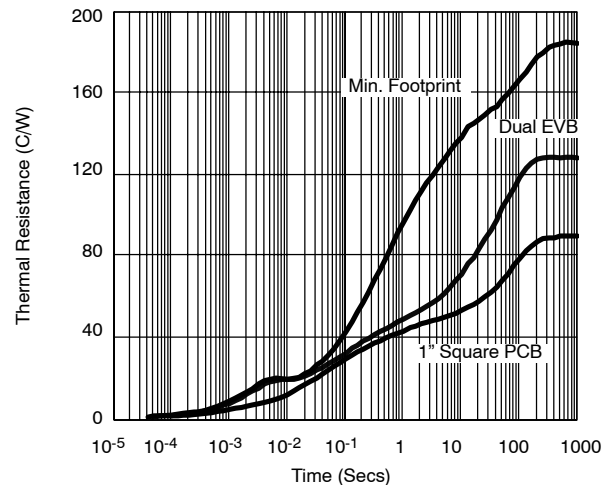
FIGURE 4. Dual 1206-8 ChipFET
