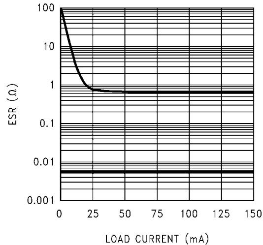
FIGURE 2. LP2985LV 4.7µF Stable ESR Range
