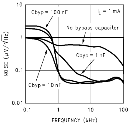
Noise Density
