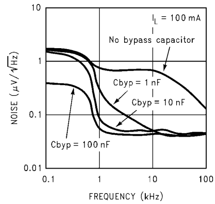
Noise Density
