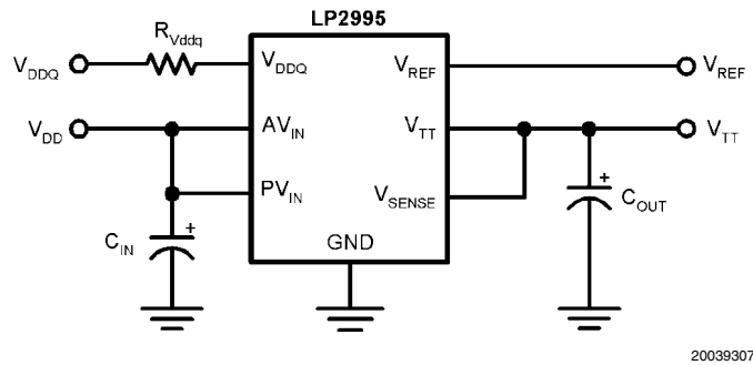
FIGURE 6. SSTL-3 Implementation
