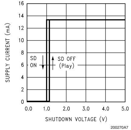
Shutdown Hysteresis Voltage V_{DD} = 5V, SD Mode = GND (SD High)
