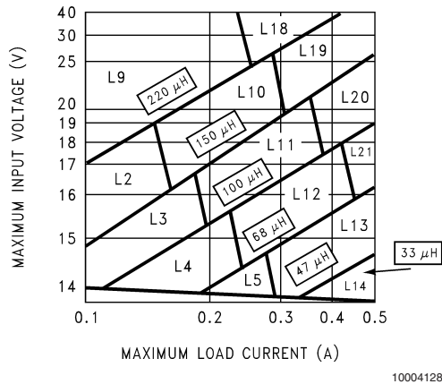
FIGURE 6. LM2674-12
