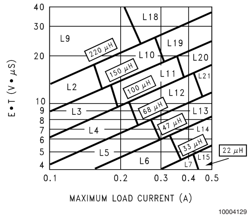
FIGURE 7. LM2674-ADJ
