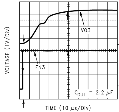
LDO3 Enable Response ( C_{OUT}=2.2\mu\text{F} )
