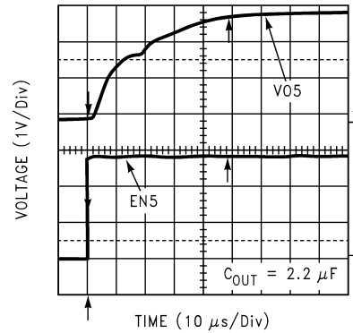
LDO5 Enable Response ( C_{OUT}=2.2\mu\text{F} )
