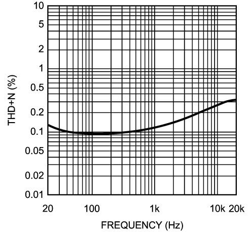
LM4859SP THD+N vs Frequency
