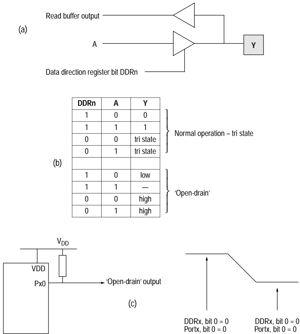
Figure 4-3 Port logic levels
