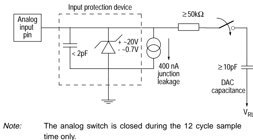
Figure 9-2 Electrical model of an A/D input pin
