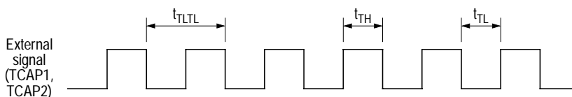
Figure 12-1 Timer relationship
