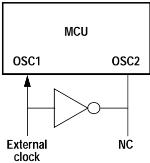
(c) External clock source connections
