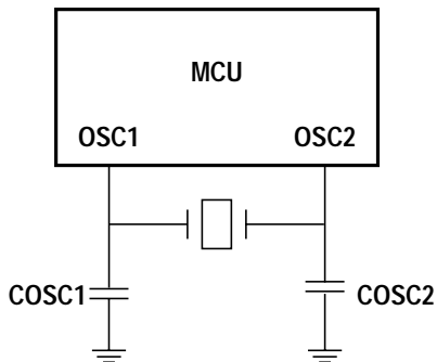
(a) Crystal/ceramic resonator oscillator connections
