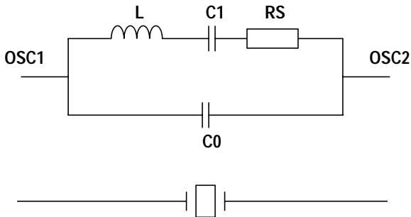
(b) Crystal equivalent circuit
