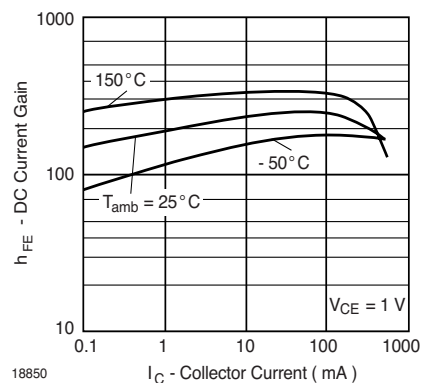
Figure 6. DC Current Gain vs. Collector Current
