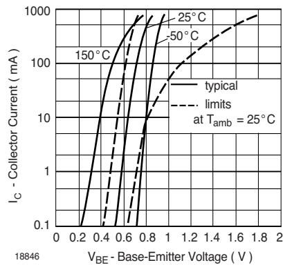
Figure 2. Collector Current vs. Base-Emitter Voltage
