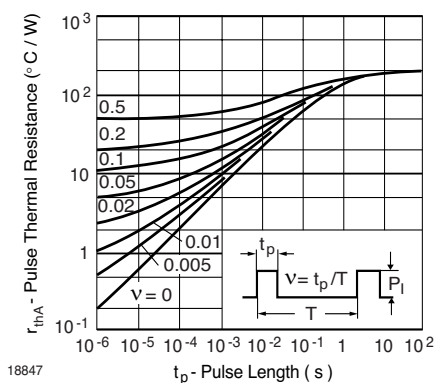
Figure 3. Pulse Thermal Resistance vs. Pulse Duration
