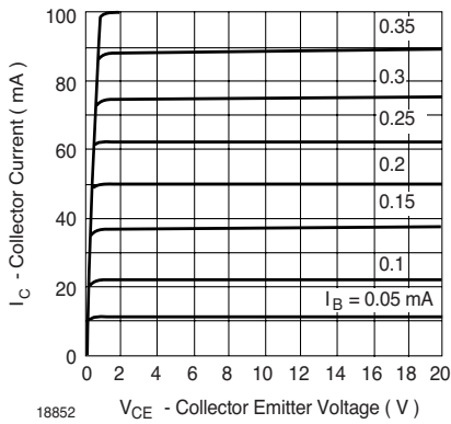
Figure 8. Collector Current vs. Collector Emitter Voltage
