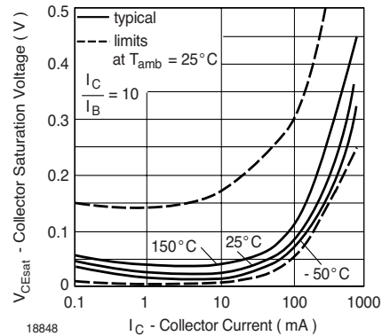
Figure 4. Collector Saturation Voltage vs. Collector Current
