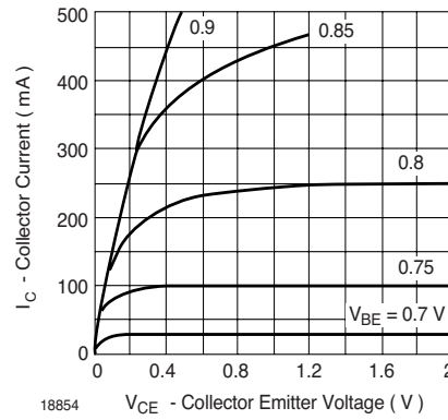
Figure 10. Collector Current vs. Collector Emitter Voltage
