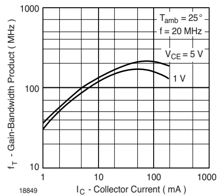
Figure 5. Gain-Bandwidth Product vs. Collector Current
