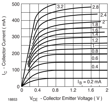
Figure 9. Collector Current vs. Collector Emitter Voltage
