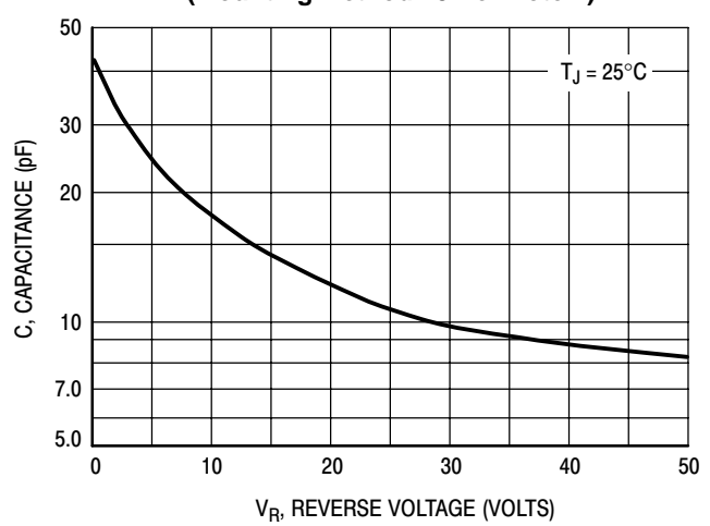
Figure 5. Typical Capacitance
