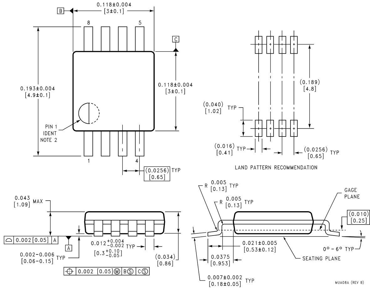
8-Lead (0.118" Wide) Molded Mini Small Outline Package Order Number LM4902MM NS Package Number MUA08A
