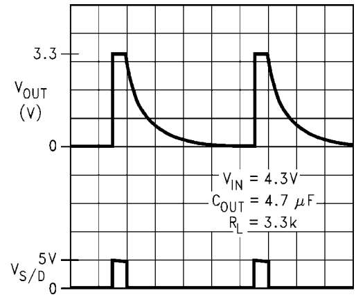
Turn-Off Waveform
