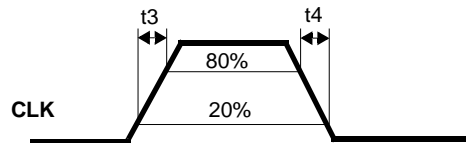
Figure 3. Rise and Fall Time Definitions: ER = 0.6 x V DD / t 3 , EF = 0.6 x V DD / t 4
