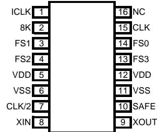
Figure 1. CY26049-36 16-Pin TSSOP (Top View)
