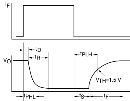
Figure 6. Switching Waveform
