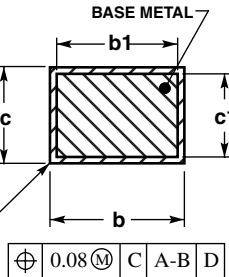
SECTION AB-AB ROTATED 90° CLOCKWISE
