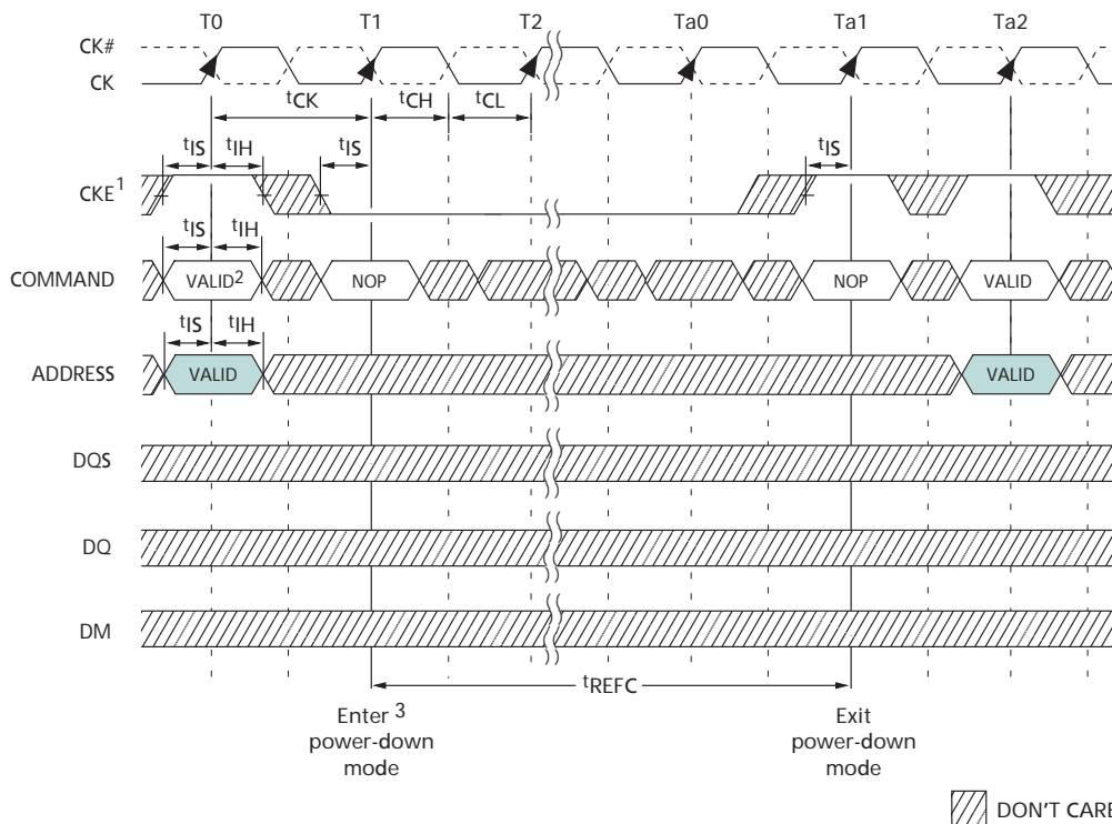
Figure 53: Power-Down Mode
