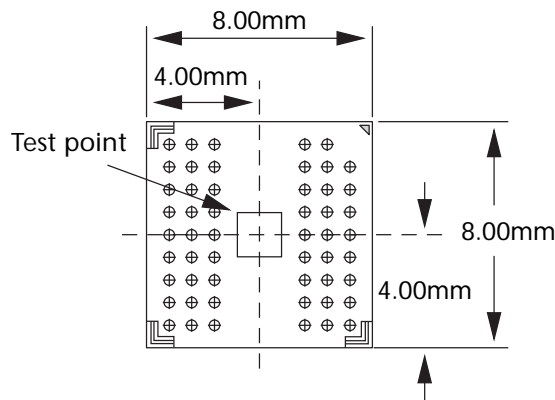
Figure 36: Example Temperature Test Point Location, 60-Ball FBGA: Top View
