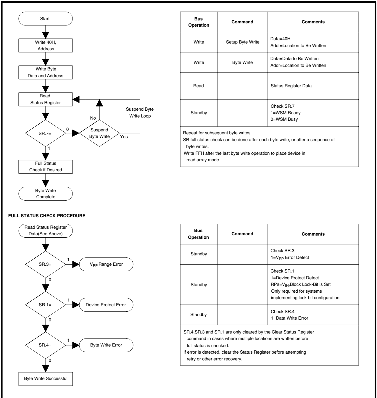
Figure 6. Automated Byte Write Flowchart
