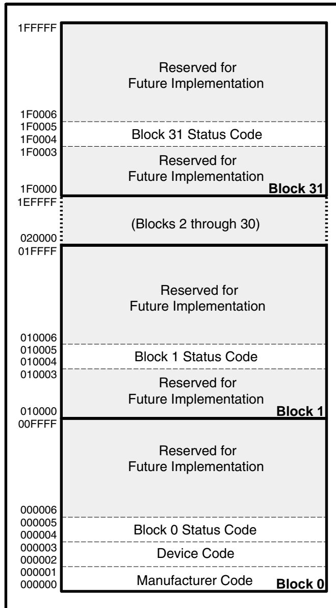
Figure 4. Device Identifier Code Memory Map
