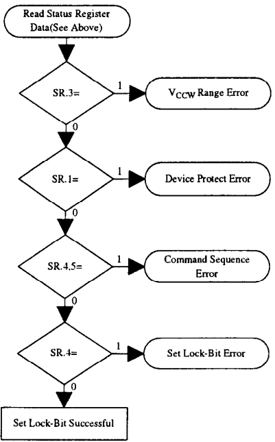
Figure 10. Set Block and Permanent Lock-Bit Flowchart
