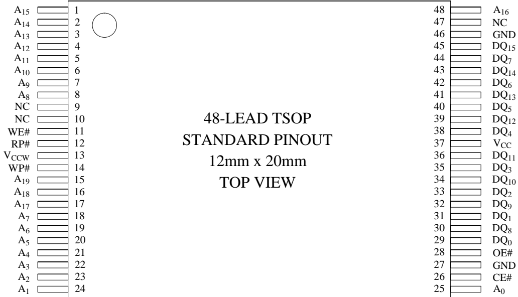
Figure 2. TSOP 48-Lead Pinout
