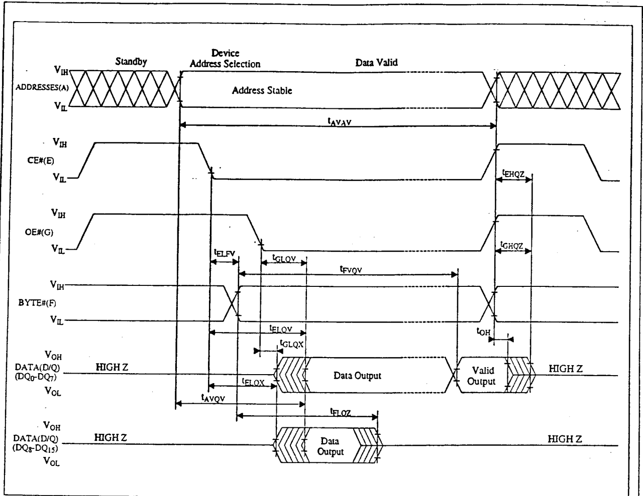
Figure 12. BYTE# timing Waveform
