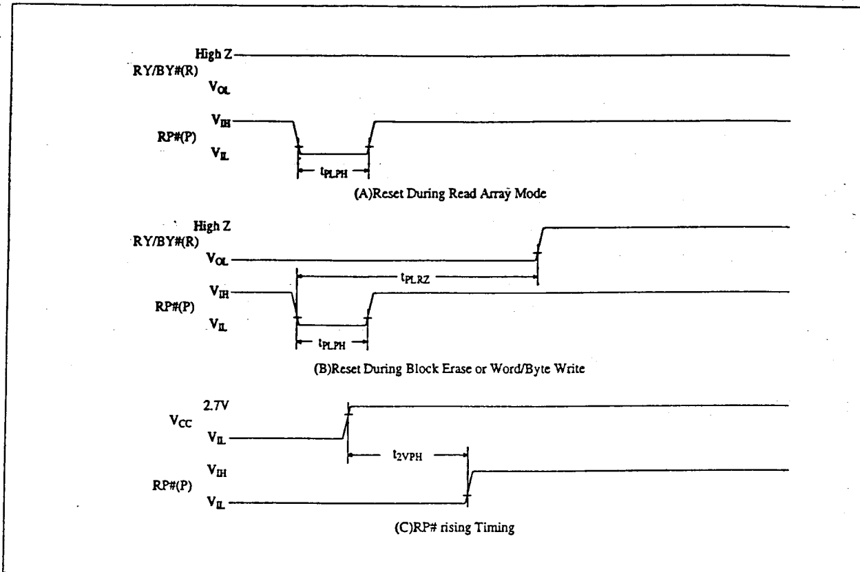
Figure 15. AC Waveform for Reset Operation
