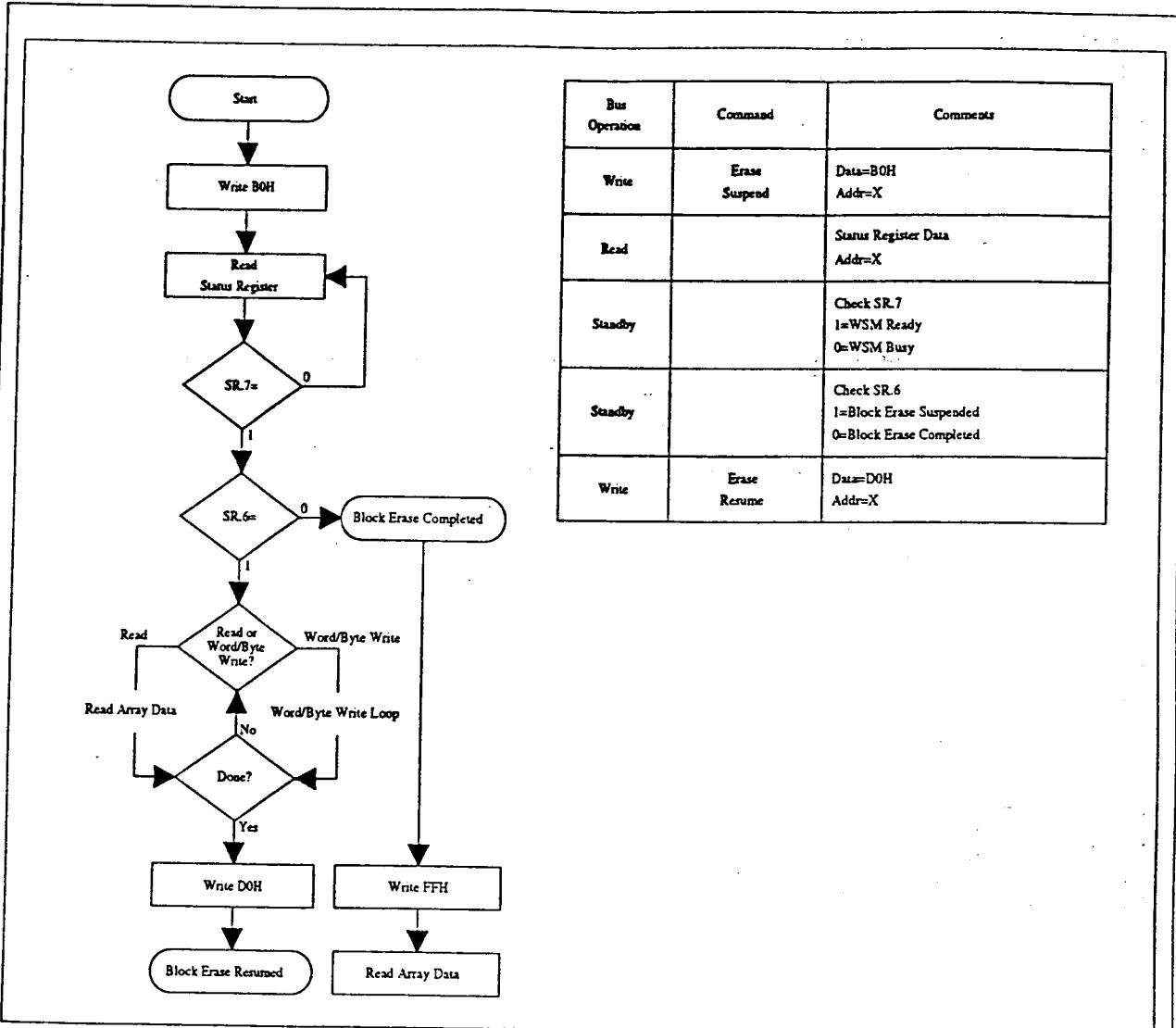
Figure 7. Block Erase Suspend/Resume Flowchart
