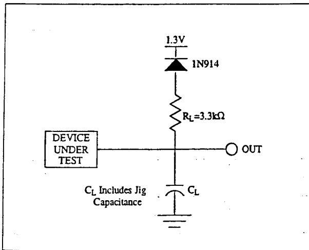
Figure 10. Transient Equivalent Testing Load Circuit
