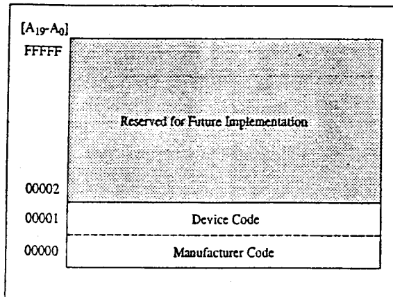
Figure 4. Device Identifier Code Memory Map
