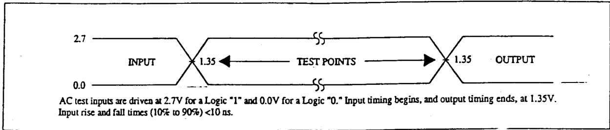
Figure 9. Transient Input/Output Reference Waveform for V_{CC}=2.7V-3.6V
