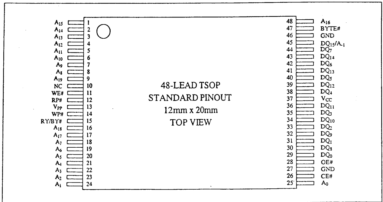
Figure 2. TSOP 48-Lead Pinout
