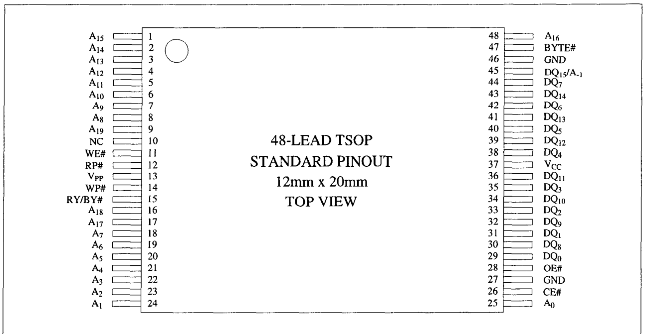
Figure 2. TSOP 48-Lead Pinout
