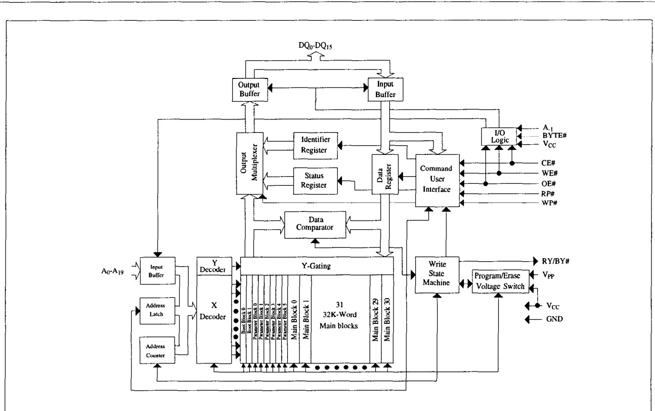
Figure 1. Block Diagram
