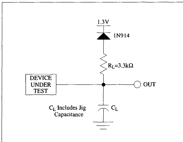
Figure 10. Transient Equivalent Testing Load Circuit
