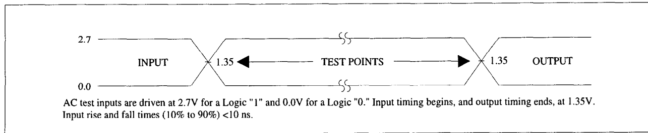
Figure 9. Transient Input/Output Reference Waveform for V_{CC}=2.7V-3.6V
