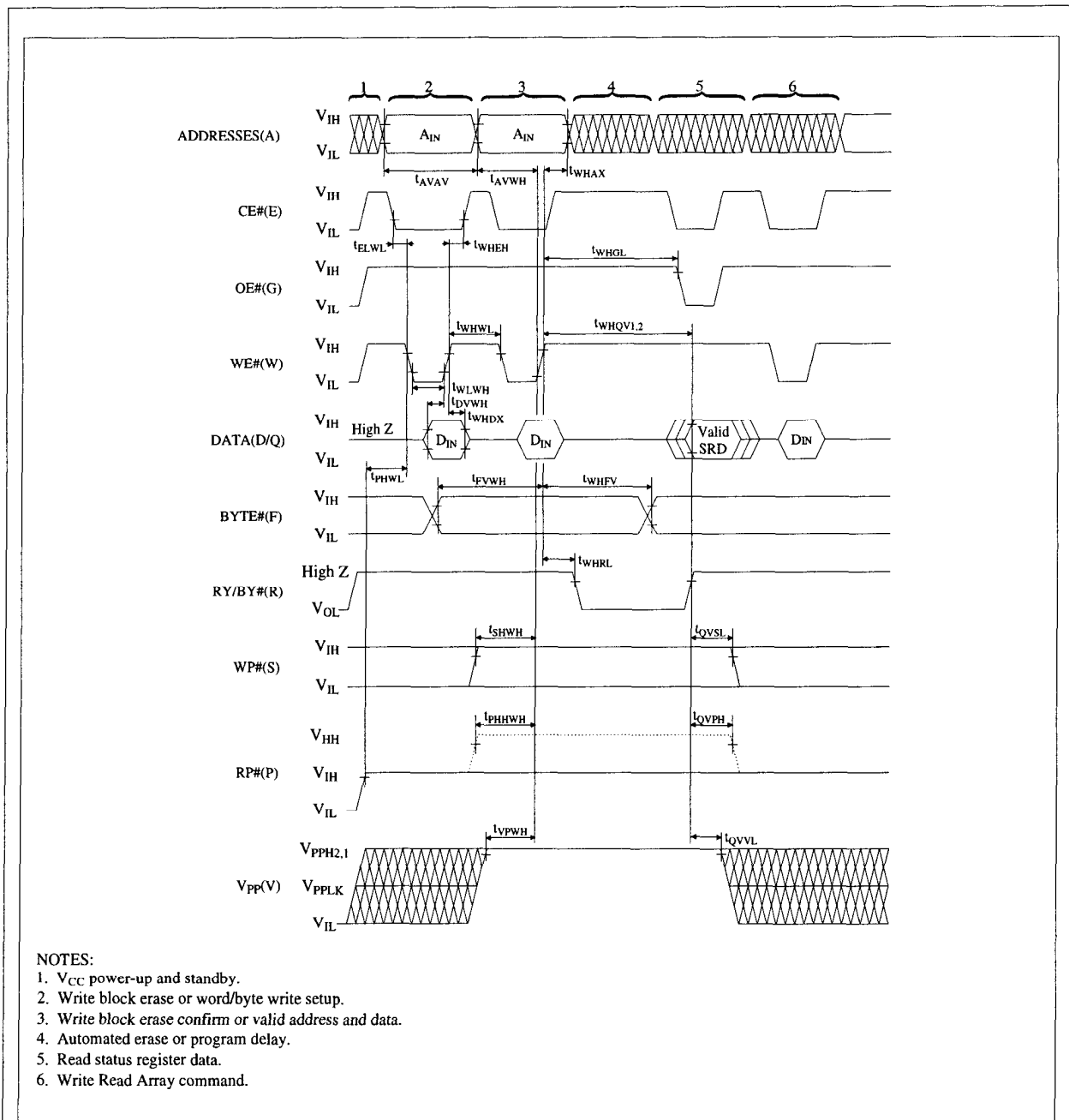
Figure 13. AC Waveform for WE#-Controlled Write Operations
