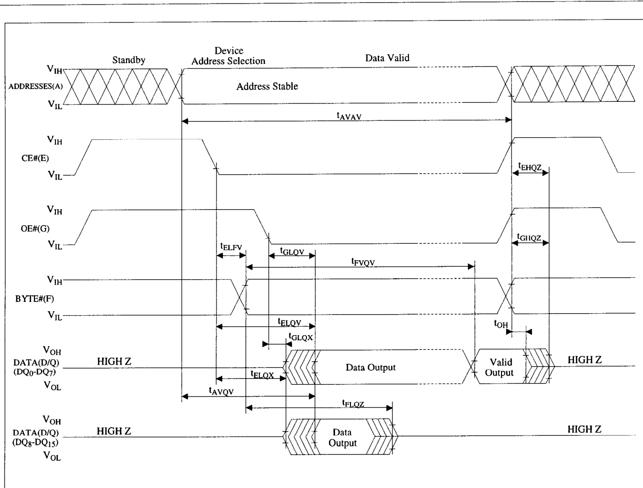
Figure 12. BYTE# timing Waveform
