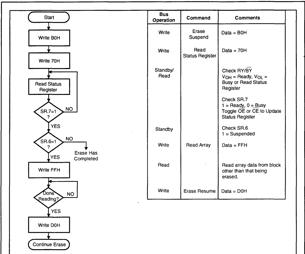
Figure 7. Erase Suspend/Resume Flowchart
