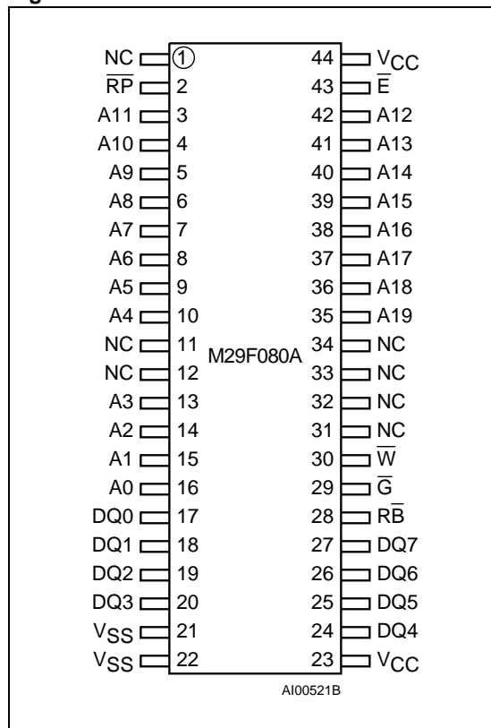
Figure 3. SO Connections
