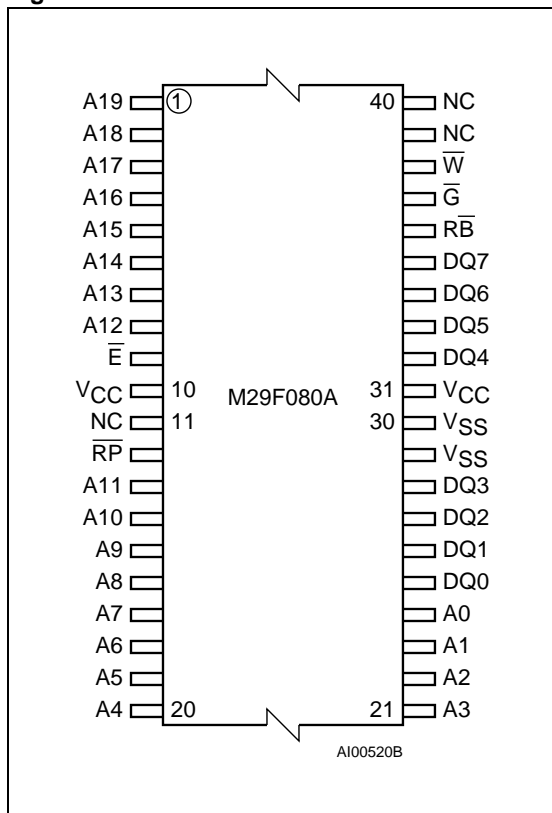
Figure 2. TSOP Connections
