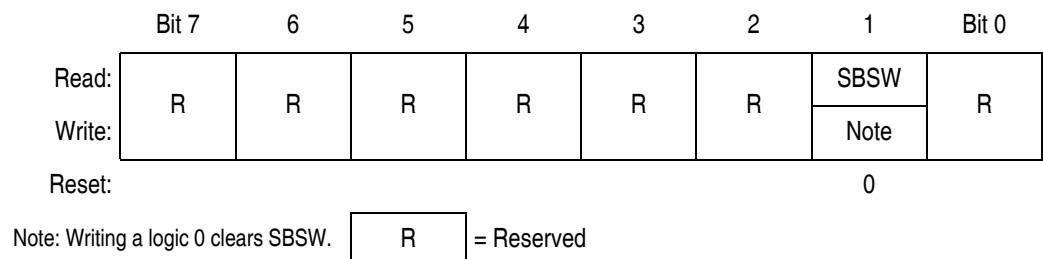
Figure 9-19. SIM Break Status Register (SBSR)
