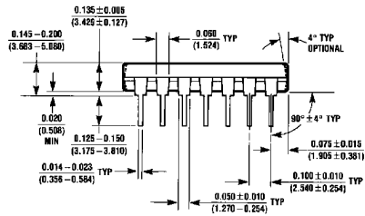
Dual-In-Line Package (N) Order Number LM565CN NS Package Number N14A
