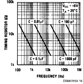
VCO Frequency
