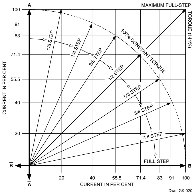
Figure 2 — Current/Displacement Vectors
