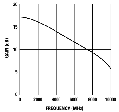
Figure 6. Gain vs. Frequency at I_d = 27 mA.
