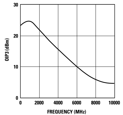
Figure 9. OIP3 vs. Frequency at I_d = 27 mA.
