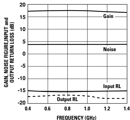
Figure 9. Gain, Noise Figure, Input and Output Return Loss Results.
